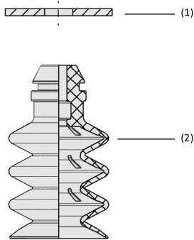
System design Bellows Suction Cups SPB3 P (3.5 folds)
