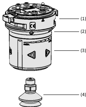
System design Electrical Vacuum Generator ECBPMi MATCH
