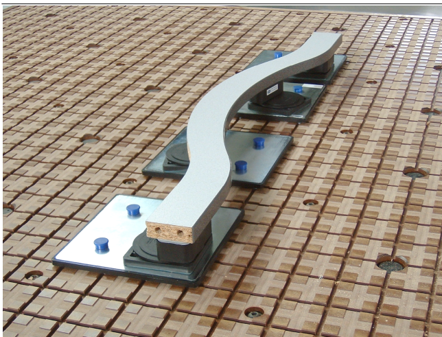
Adapter-Plates ISAP-R with Mono-Base and suction cups for clamping curved workpieces
