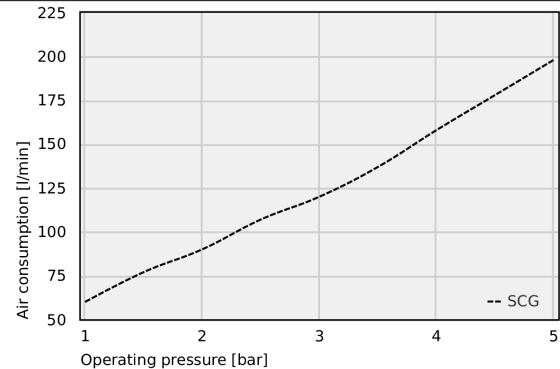
Air consumption
